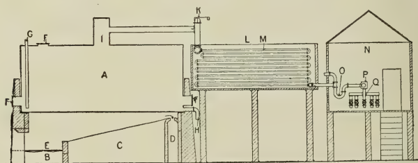
FIG. 106.—Plant for Refining Petroleum.
